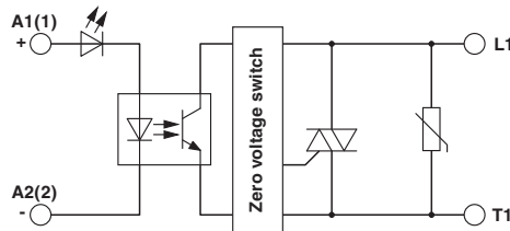
Block diagram
