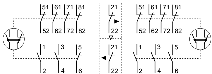
104S-C30⊗010C...C85⊗010C
