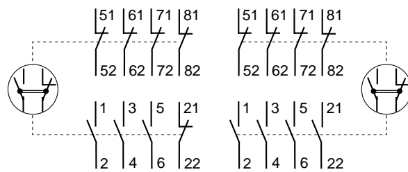
104S-C09⊗010C...C23⊗010C
