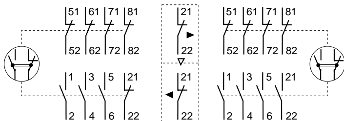
104S-C09⊗012C...C23⊗012C
